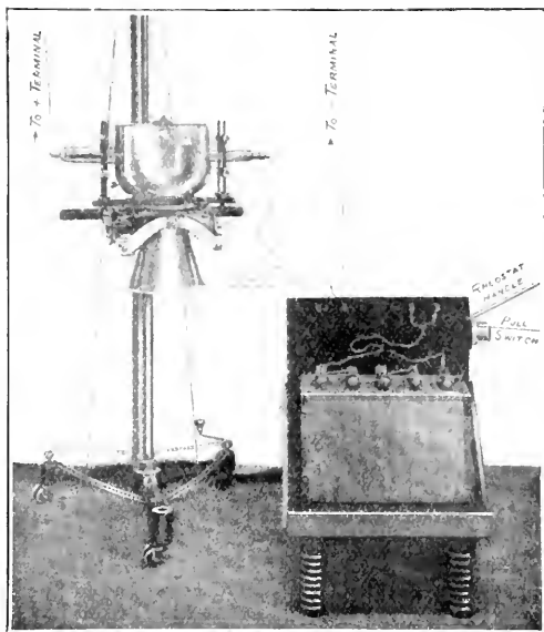
FIG. 34.—Complete Coolidge X-ray equipment in position. (B.T.H.)
